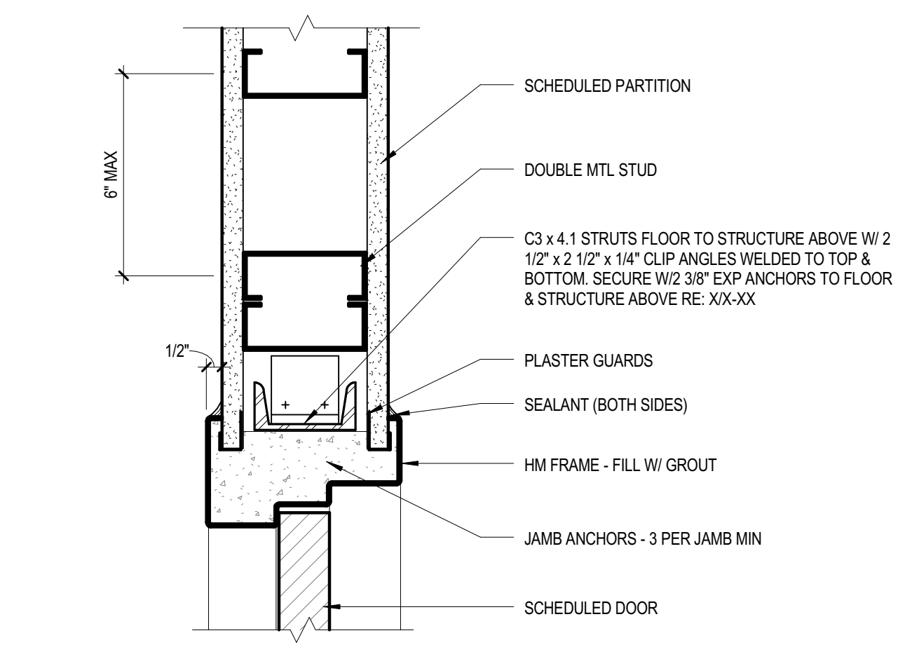
06 JAMB DETAIL 3" = 1'-0" @ DOUBLE EGRESS DOORS C1020.01-1D
