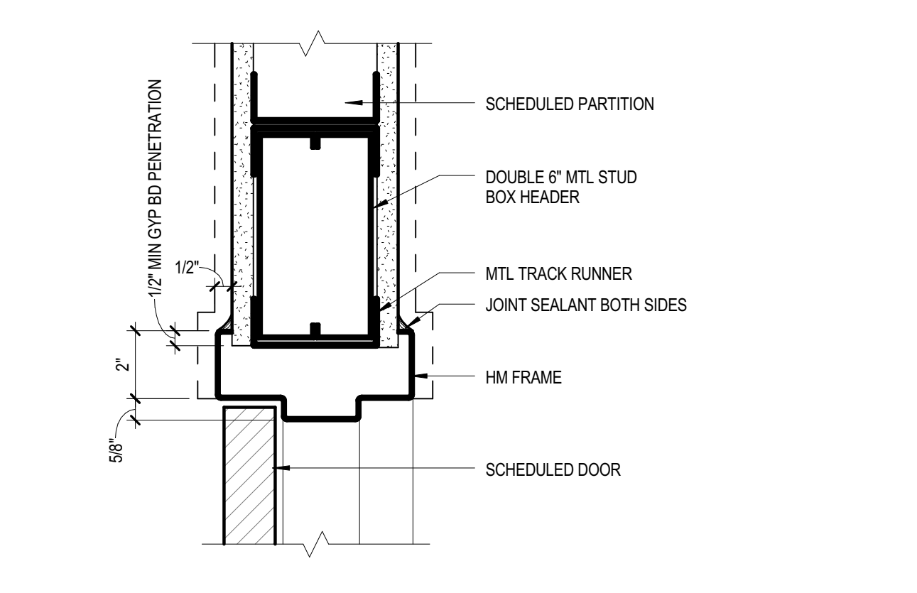
05 HEAD DETAIL 3" = 1'-0" @ TYP RATED/ NON-RATED DOORS C1020.01-1B
