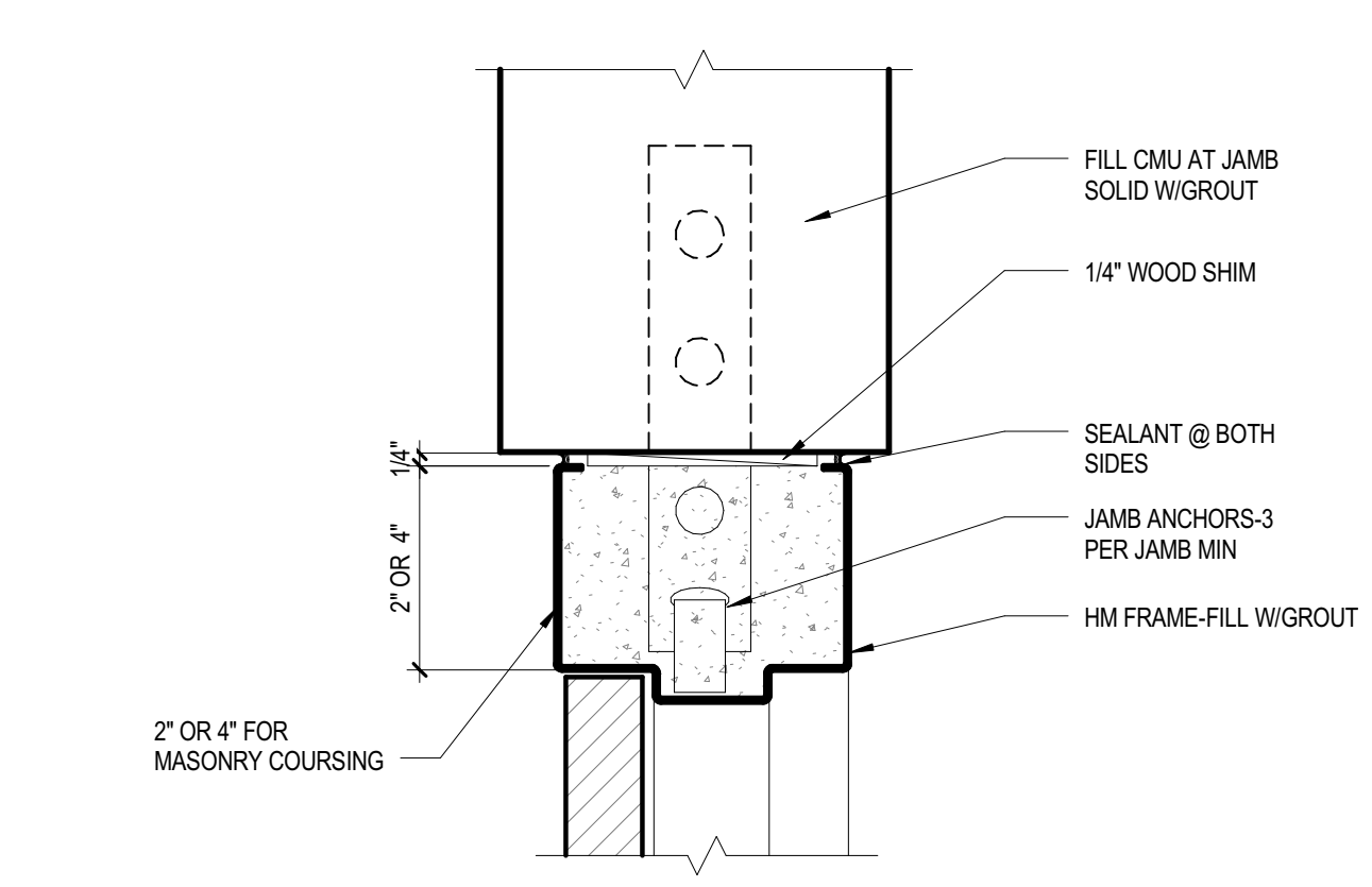
10 JAMB DETAIL 3" = 1'-0" @ METAL FRAME IN CMU PARTITION C1020.01-1F
