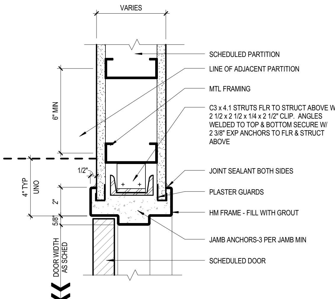
13 JAMB DETAIL 3" = 1'-0" @ PAIR OF DOORS C1020.01-1F
