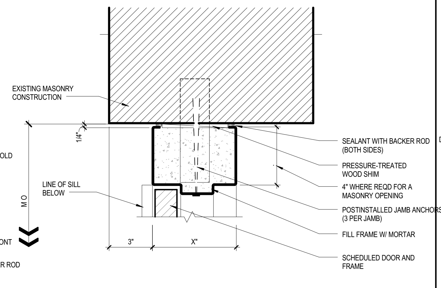
04 JAMB DETAIL 3" = 1'-0" @ EXT SWINGING DOOR IN MASONRY B2030.01-2A
