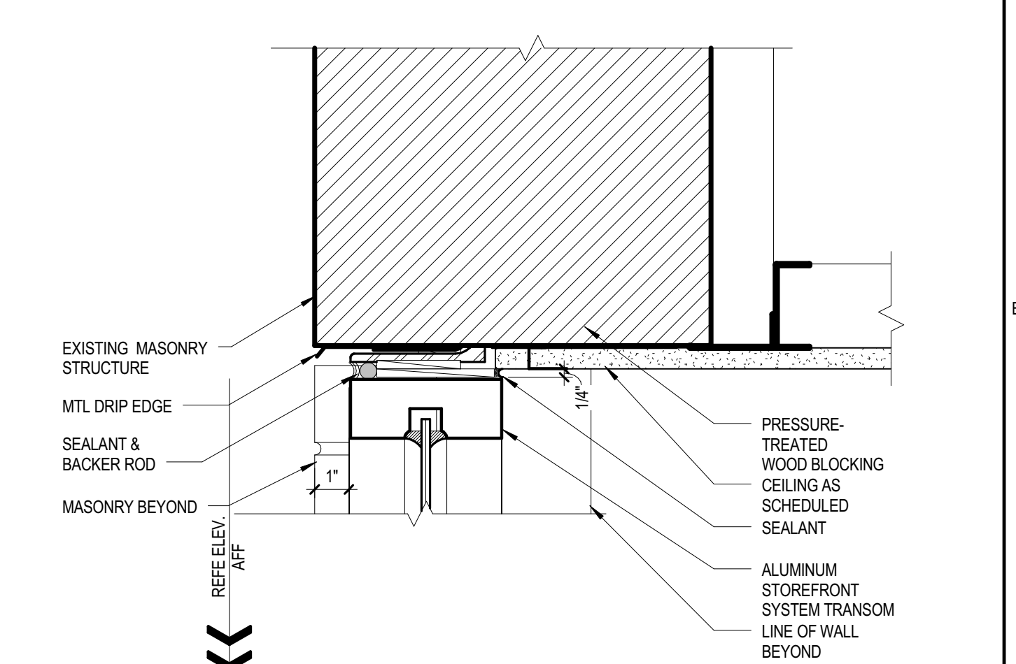
02 HEAD DETAIL 3" = 1'-0" @ ALUM STOREFRONT SYSTEM TRANSOM B2030.02-1C
