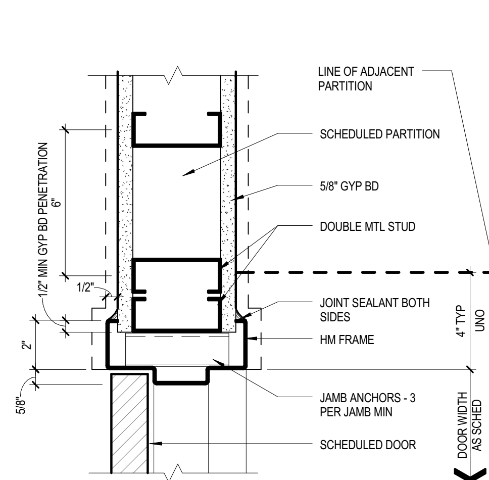
12 JAMB DETAIL 3" = 1'-0" @ TYP RATED/ NON-RATED DOOR C1020.01-1A
