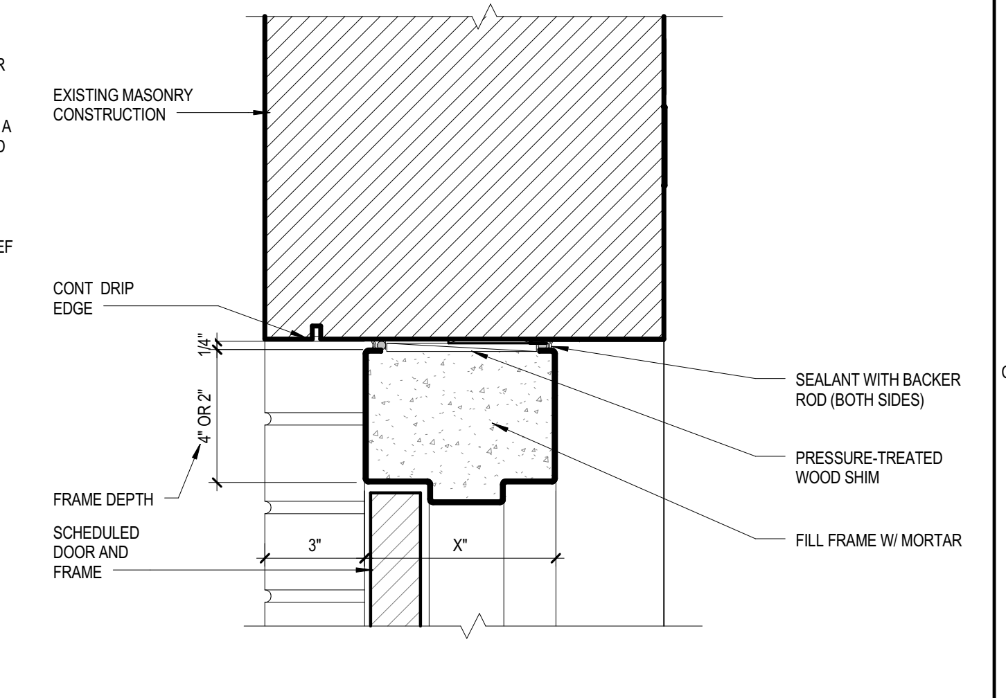
03 HEAD DETAIL 3" = 1'-0" @ TYP EXT SWINGING DOOR B2030.01-1C
