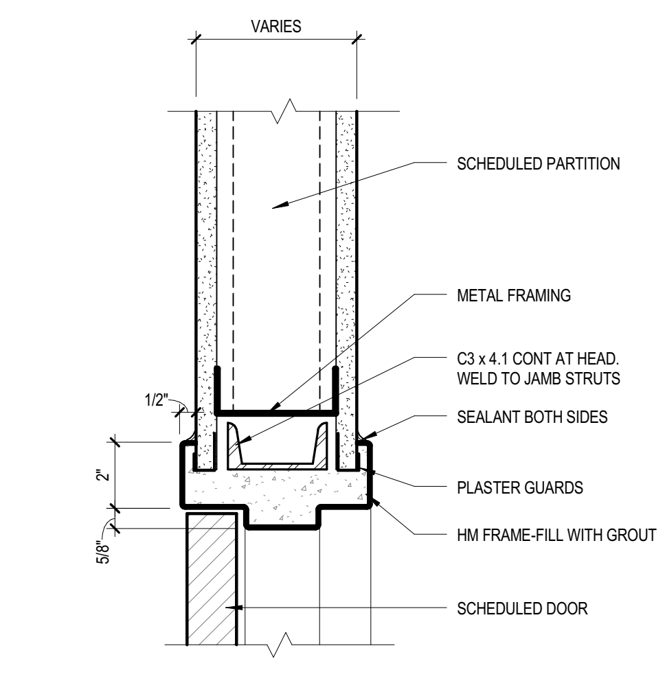
09 HEAD DETAIL 3" = 1'-0" @ PAIR OF DOORS C1020.01-1G
