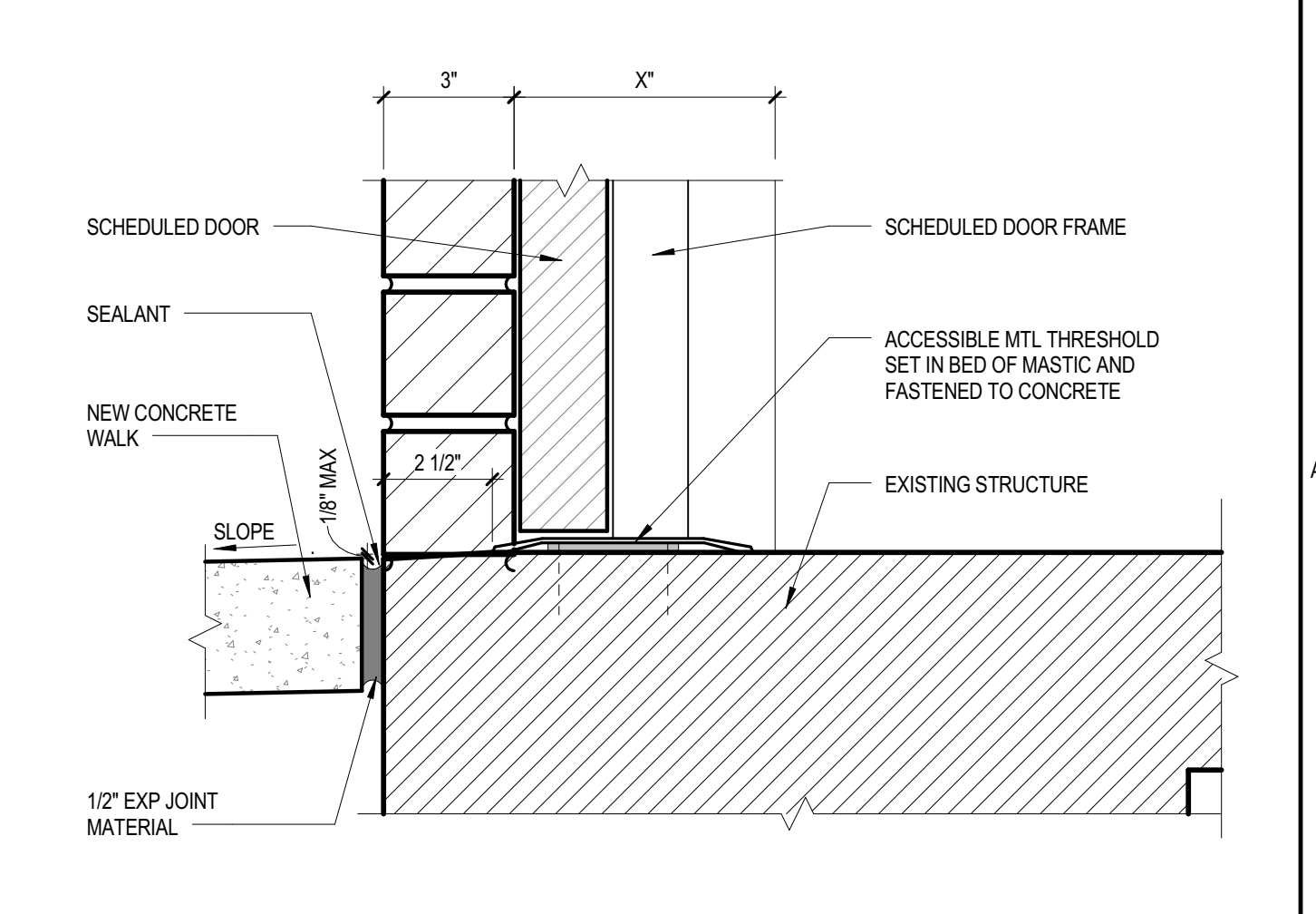
01 THRESHOLD DETAIL 3" = 1'-0" @ EXTERIOR SWINGING DOORS B2030.01-1A
