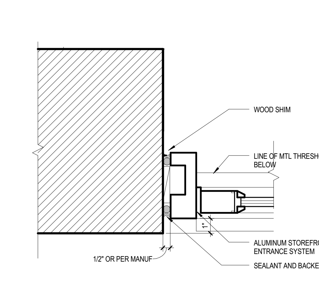
08 JAMB DETAIL 3" = 1'-0" @ ALUM STOREFRONT DOOR B2030.02-1B
