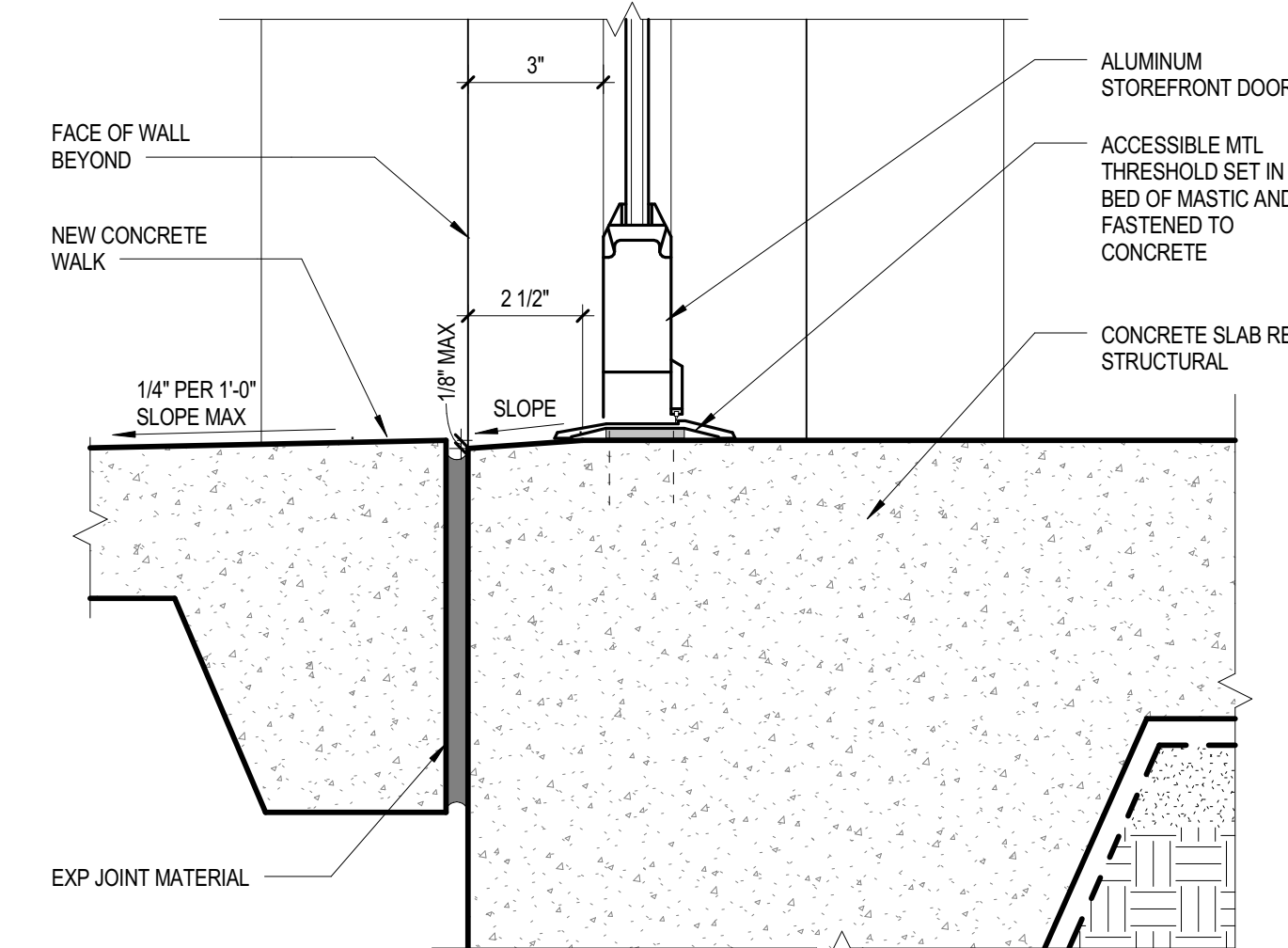
07 SILL DETAIL 3" = 1'-0" @ ALUM STOREFRONT DOOR B2030.01-1A
