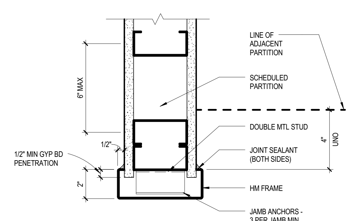
11 JAMB / HEAD DETAIL 3" = 1'-0" @ DOUBLE ACTING DOOR AND CASD OPENING C1020.01-1B
