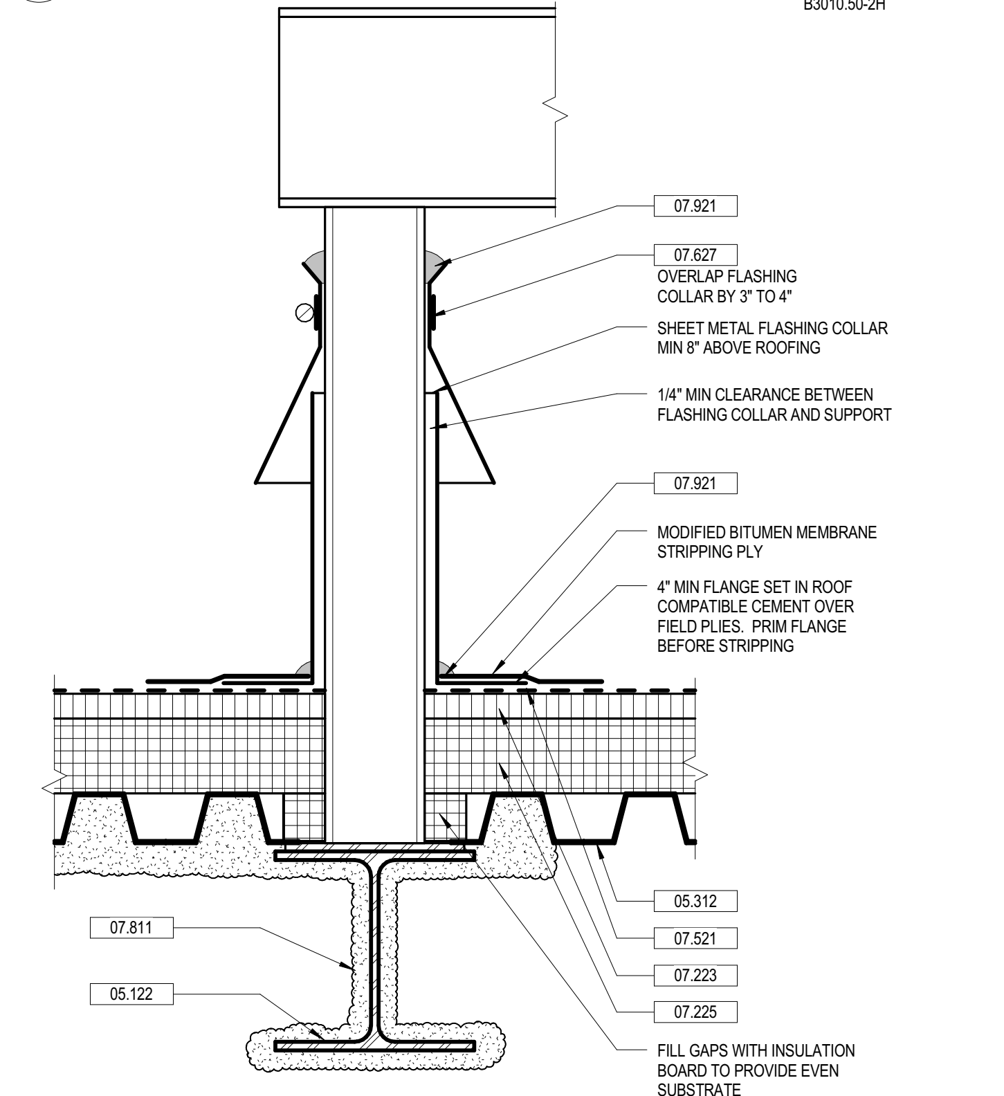
07 MBR SECTION DETAIL 3" = 1'-0" EQUIPMENT SUPPORT STAND AND RAIN COLLAR PENETRATION B3010.50-2G
