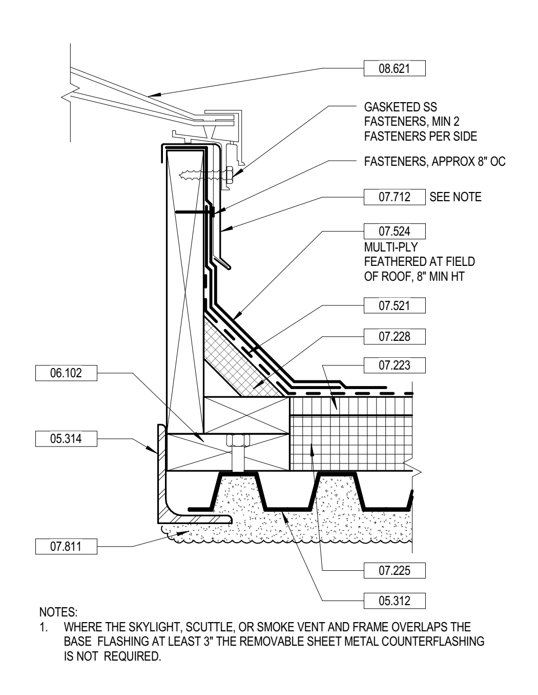
10 MBR SECTION DETAIL 3" = 1'-0" SKYLIGHT, SCUTTLE AND SMOKE VENT B3010.50-2J
