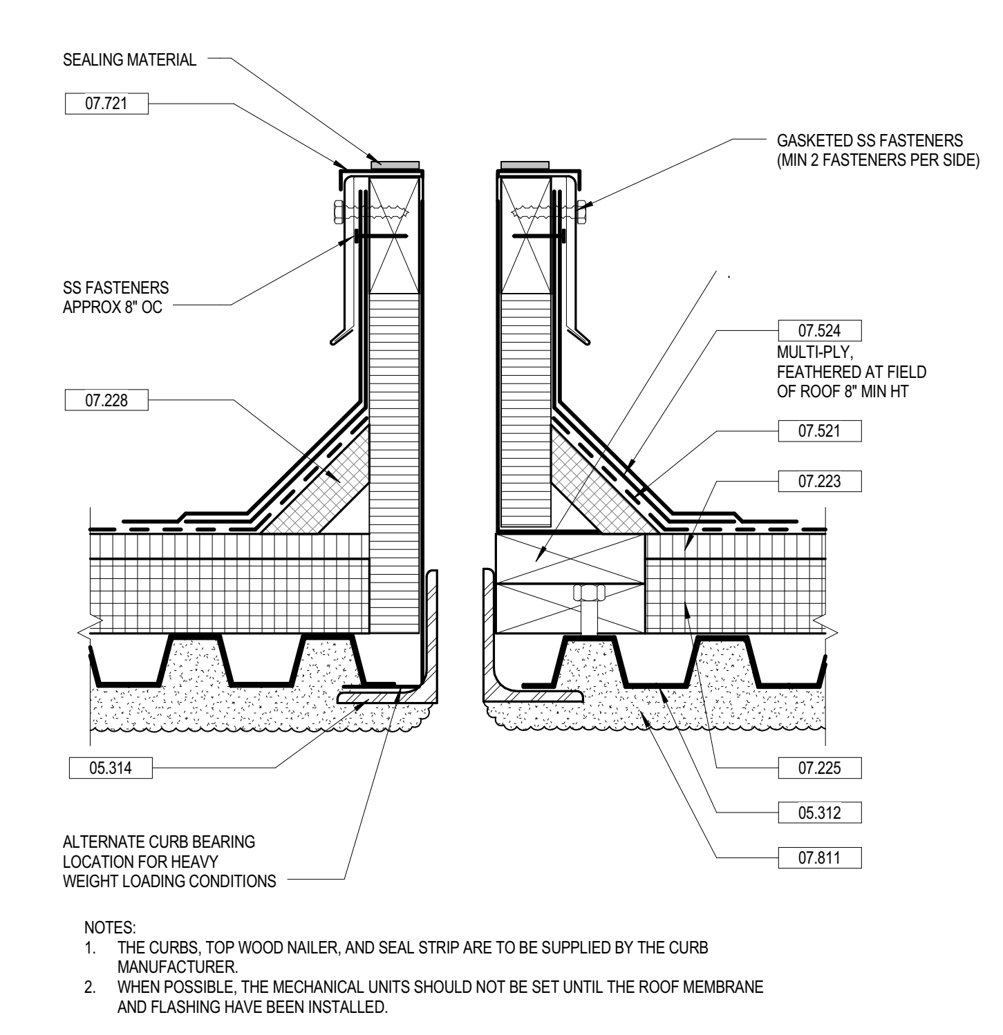
08 MBR SECTION DETAIL 3" = 1'-0" RAISED PRE-FABRICATED METAL CURB B3010.50-2H
